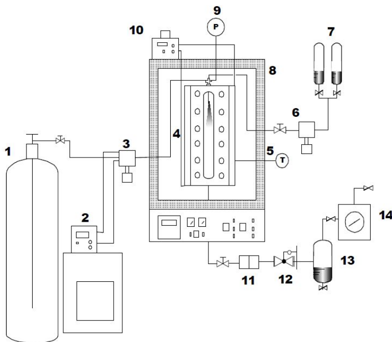
Figure 2. Schematic diagram of the ASES apparatus
