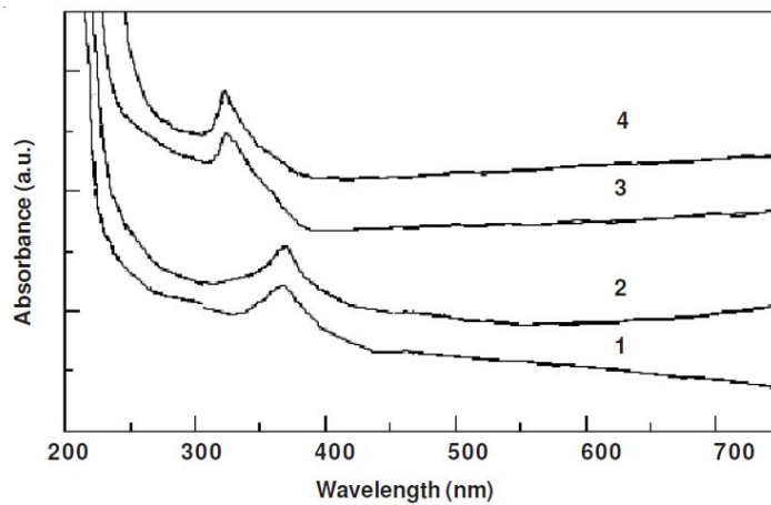
Figure 4. UV-visible absorption spectra of samples
