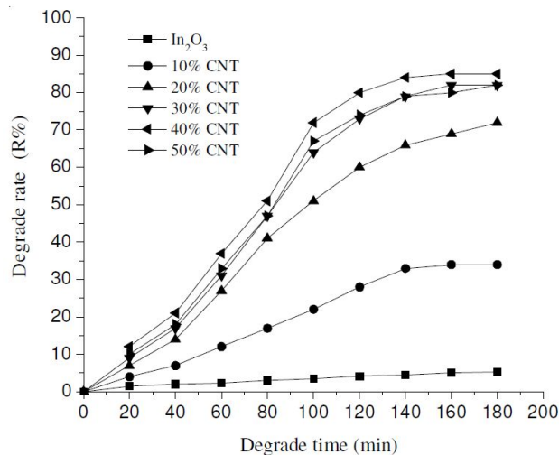
Figure 5. Degradation rate curves of CNT/ \text{In}_2\text{O}_3 for methylene blue
