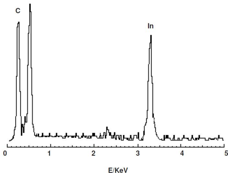
Figure 3. EDS of the sample 3.
