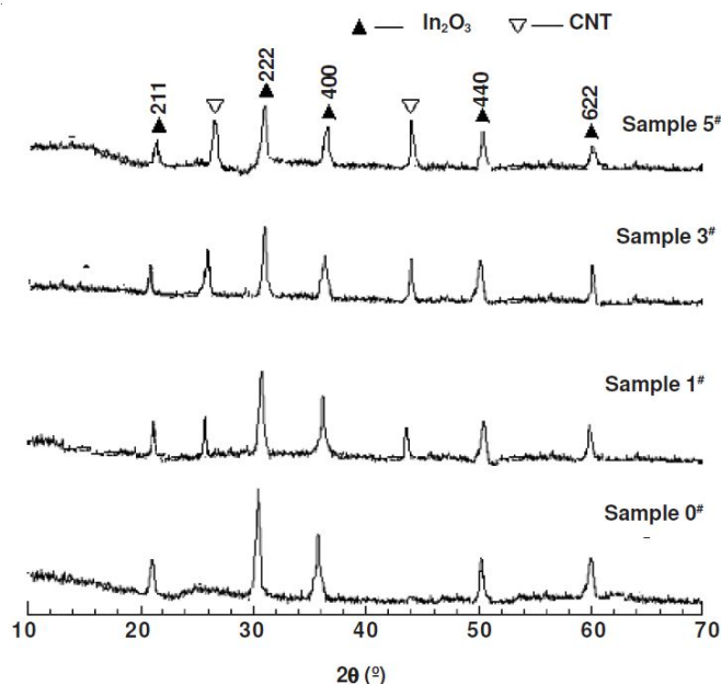
Figure 1. XRD patterns of the samples
