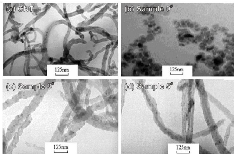
Figure 2. TEM images of the samples
